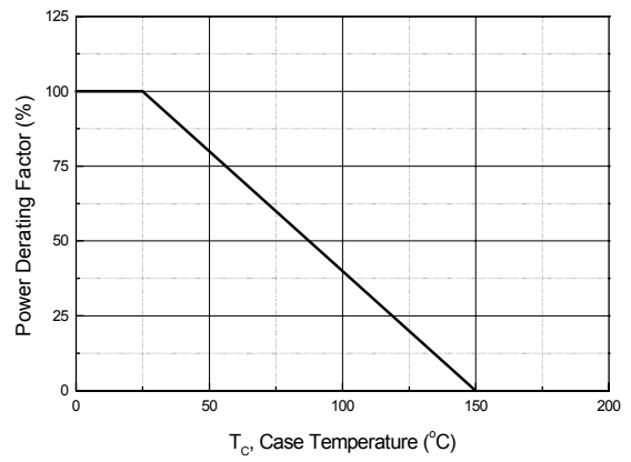
Fig 8. Power Derating Curve
